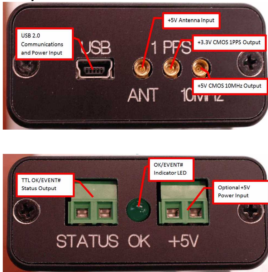
Figure 2.3 Major connections to LC-XO-PLUS enclosure
